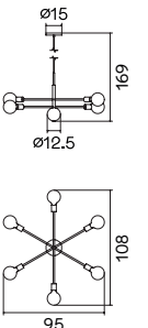
Ref. 802/6 PT Latão escovado/Preto areado EN Brushed brass/Sand black 6 x E27 49033/05/62 Ø12.5 cm (B) Ø15 cm L108*W95*H169 cm
