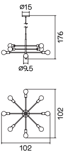
Ref. 802/8 PT Latão escovado/Preto areado EN Brushed brass/Sand black 8 x E27 49032/05/62 Ø9.5 cm (B) Ø15 cm L102*W102*H176 cm
