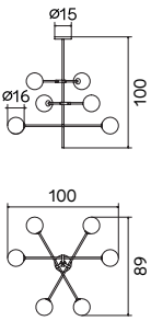
Ref. 741/6 PT Latão escovado EN Brushed brass 6 x G9 (B) Ø15 cm (G) Ø16 cm L100*W89*H100 cm
