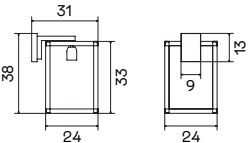
Ref. 667/AP PT Preto areado EN Sand black 1 x E27 (49033/05/62 Ø12.5 cm) (B) L13*W9 cm (L) L24*W24*H33 cm L31*W24*H38 IP20
