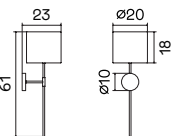
Ref. 744/AP PT Latão escovado EN Brushed brass 1 x E27 (B) Ø10 cm (A) 028 Ø20*H18 cm L23*W20*H61 cm
