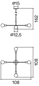
Ref. 802/4 PT Latão escovado/Preto areado EN Brushed brass/Sand black 4 x E27 49033/05/62 Ø12.5 cm (B) Ø15 cm L108*W108*H162 cm
