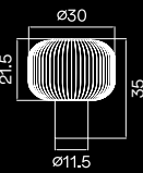
Ref. 101195191 PT Travertino/Vidro EN Travertine/Glass 1 x E27 (B) ø11.5 cm (V) ø30*H21.5 cm H t 35 cm
