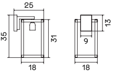
Ref. 667/APP PT Preto areado EN Sand black 1 x E27 (49032/05/62 Ø9.5 cm) (B) L13*W9 cm (L) L18*W18*H31 cm L25*W18*H35 cm IP20
