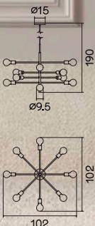
Ref. 802/12 PT Latão escovado/Preto areado EN Brushed brass/Sand black 12 x E27 49032/05/62 Ø9.5 cm (B) Ø15 cm L102*W102*H190 cm
